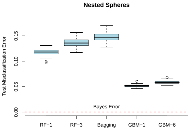
FIGURE 15.2. The results of 50 simulations from the “nested spheres” model in \mathbb{R}^{10} . The Bayes decision boundary is the surface of a sphere (additive). “RF-3” refers to a random forest with m = 3 , and “GBM-6” a gradient boosted model with interaction order six; similarly for “RF-1” and “GBM-1.” The training sets were of size 2000, and the test sets 10,000.
