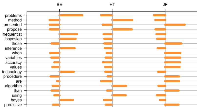
FIGURE 18.10. Abstracts example: top 20 scores from nearest shrunk centroids. Each score is the standardized difference in frequency for the word in the given class (BE, HT or JF) versus all classes. Thus a positive score (to the right of the vertical grey zero lines) indicates a higher frequency in that class; a negative score indicates a lower relative frequency.
