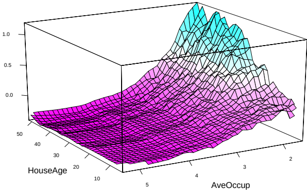
FIGURE 10.16. Partial dependence of house value on median age and average occupancy. There appears to be a strong interaction effect between these two variables.
