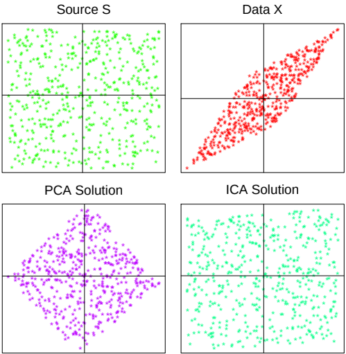
FIGURE 14.38. Mixtures of independent uniform random variables. The upper left panel shows 500 realizations from the two independent uniform sources, the upper right panel their mixed versions. The lower two panels show the PCA and ICA solutions, respectively.
